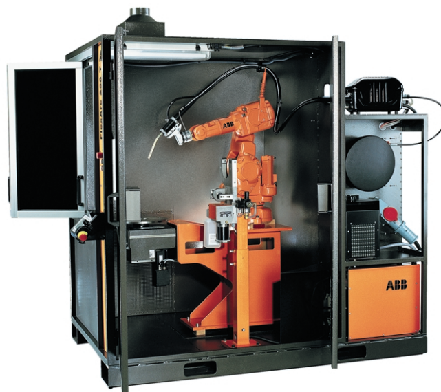
2 FlexArc Compact is a self-contained, skid-mounted, welding cell, containing an IRB 140 robot and a cell management system. It provides immediate flexibility by eliminating bottlenecks and facilitating rapid change-over between jobs.
